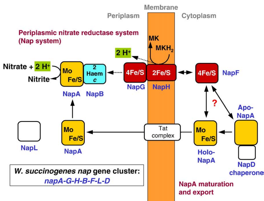
Fig. 3. The respiratory Nap system of W. succinogenes . Nitrate is reduced by a periplasmic NapAB complex that is likely to be reduced by the membrane-bound menaquinol dehydrogenase complex NapGH (cf. Fig. 4). The molybdenum cofactor (Mo) and the iron-sulfur centre of NapA are attached in the cytoplasm by specific maturation systems prior to Holo-NapA export by the twin-arginine translocation (Tat) complex. The chaperone NapD is required to coordinate maturation and export of NapA. The cytoplasmic interaction between NapF and NapA has not been shown experimentally in W. succinogenes . See text for details.
