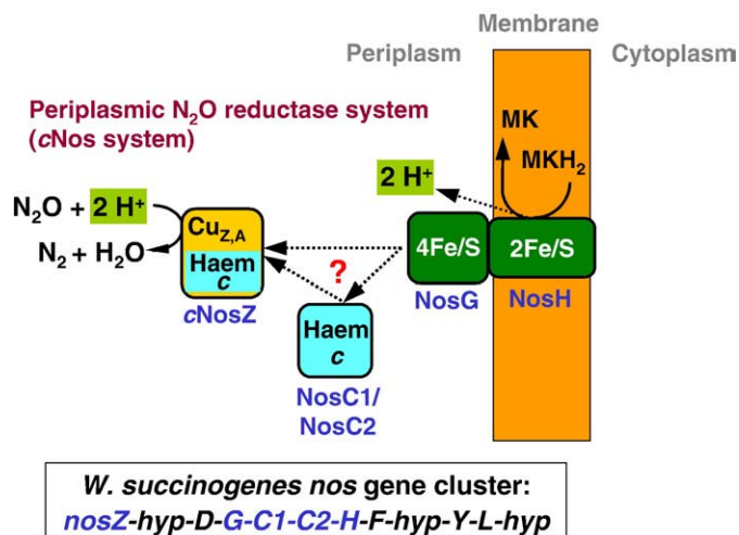
Fig. 6. Model of the respiratory cNos system of W. succinogenes . The function of the menaquinol-oxidizing NosGH complex and the electron transfer pathway to cytochrome c nitrous oxide reductase (cNosZ) via NosC1 and NosC2 is speculative. The nosF , -Y , and -D genes encode a membrane-bound ABC transporter involved in the maturation of the Nos system [96]. The hypothetical open reading frame ( hyp ) situated between nosZ and nosD in W. succinogenes is conserved in all Epsilonproteobacteria listed in Table 1 whereas those located downstream of nosF and nosL are not present throughout. Note that napL is absent from the nos clusters in C. concisus and C. curvus . Cu Z,A , binuclear Cu A and tetranuclear Cu Z centres of cNosZ.
