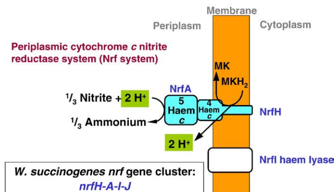
Fig. 5. The respiratory Nrf system of W. succinogenes . NrfHA is a membrane-bound menaquinol:nitrite oxidoreductase complex. Protons deriving from menaquinol oxidation are liberated on the periplasmic side of the membrane thus rendering the overall reaction electroneutral (see protons with green background). NrfI is a cytochrome c haem lyase that specifically attaches haem to the CXXCK haem c binding motif of NrfA [83]. The nrfI gene is absent in nrf gene clusters that encode a NrfA homolog with five CXXCH haem c binding motifs (Table 1).
